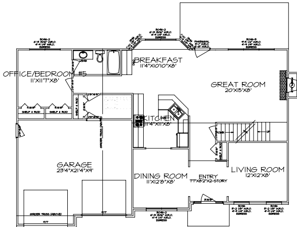
FIRST FLOOR PLAN A-5 SCALE: 1/4"=1'-0"
