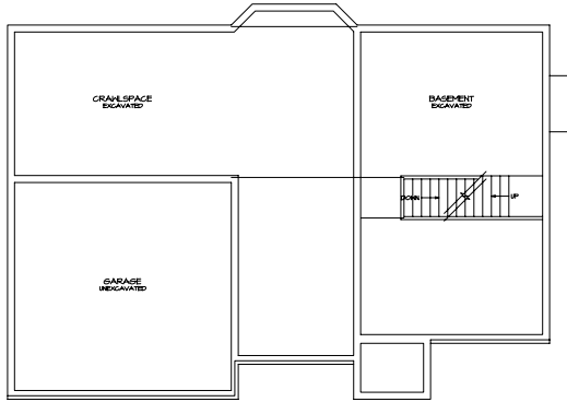
FOUNDATION PLAN A-4 SCALE: 1/4"=1'-0"
