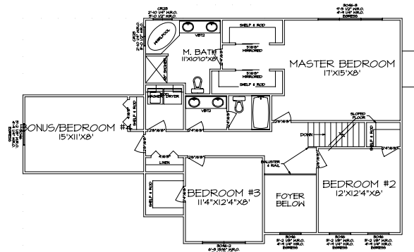
SECOND FLOOR PLAN A-5 SCALE: 1/4"=1'-0"
